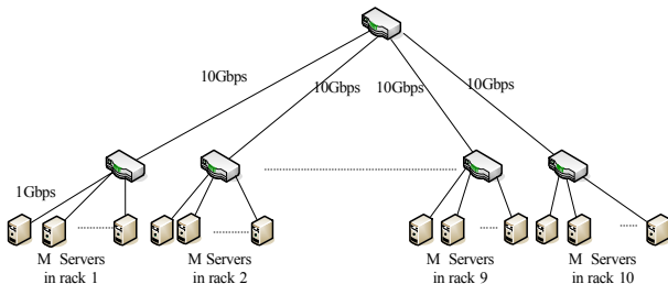
Fig. 7: The Data Center topology
