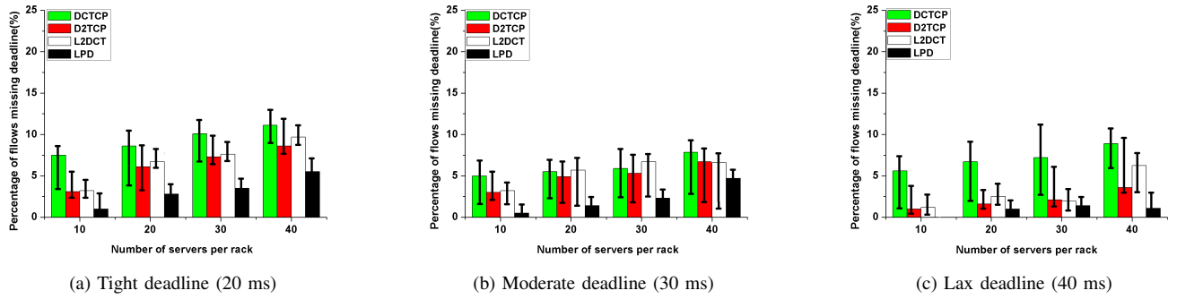
Fig. 10: Deadline missing rate for random flows (Pareto Distribution), in DCTCP, D 2 TCP, L 2 DCT and LPD-e
