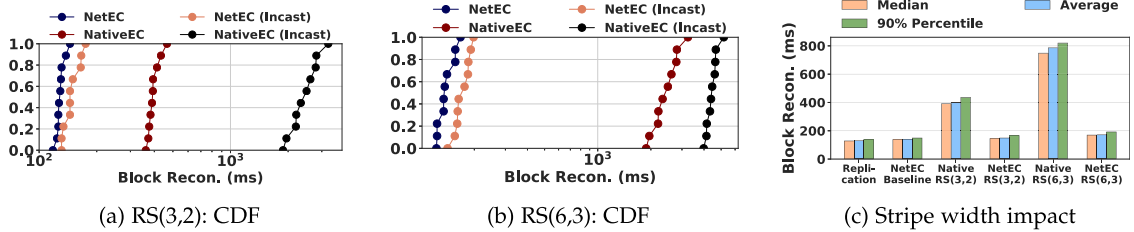
Fig. 6. Degraded read latency.
