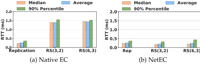
Fig. 7. Incast level reflected by RTT.
