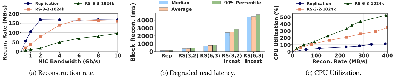
Fig. 2. Case studying of current EC in HDFS indicates considerable performance overheads.
