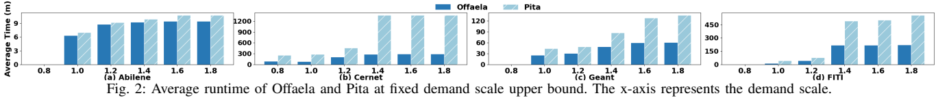
Fig. 2: Average runtime of Offaela and Pita at fixed demand scale upper bound. The x-axis represents the demand scale.
