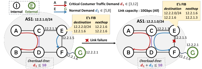
Fig. 1: Traffic load distribution under different failure scenarios
