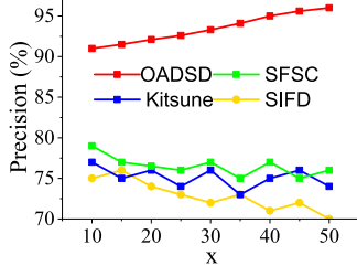
Fig. 19. Different x .
