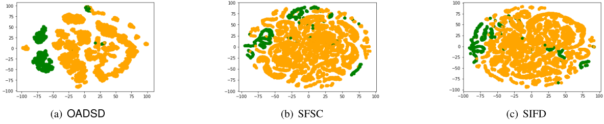
Fig. 11. The T-SNE [41] visualization of different feature extraction method under CICIDS data set. The green dots represents malicious traffic, the yellow dots represents normal traffic.
