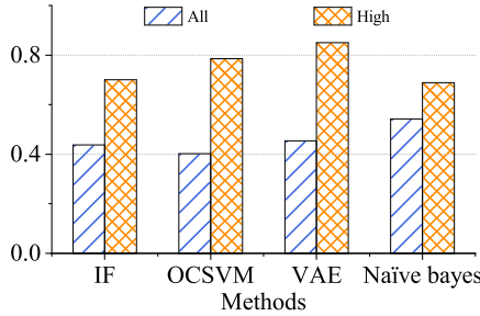
Fig. 2. F1-score of different feature set.
